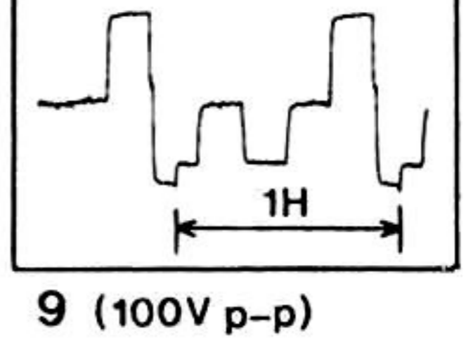
9 (100Vp-p)
